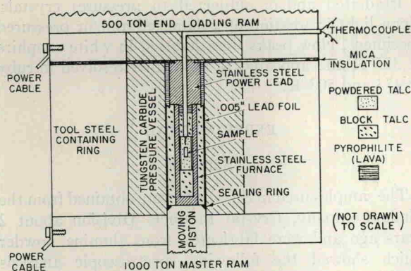
FIG. 1. Diagram of high-pressure cell and furnace assembly.
